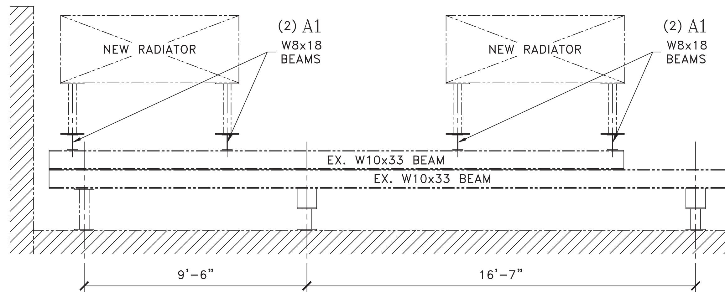
SECTION B-B
