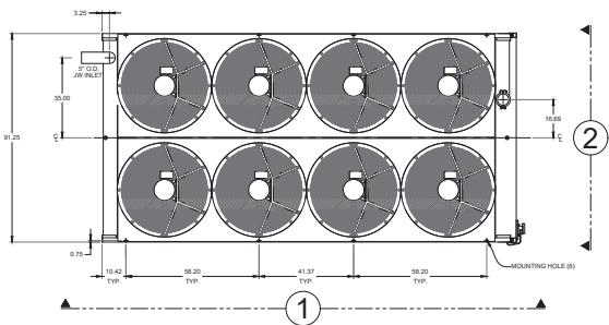
A DETAILS - HORIZONTAL REMOTE RADIATOR SCALE: NONE
