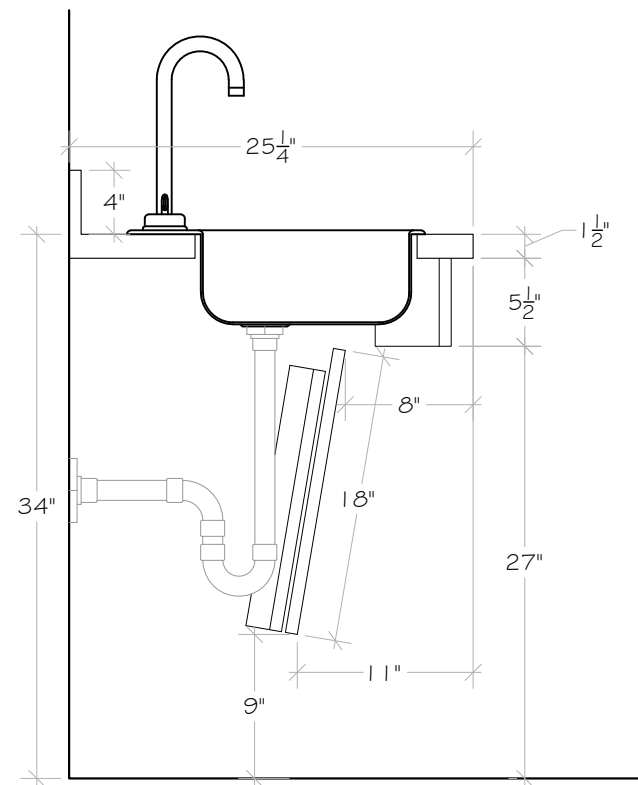
VERT. SECTION 02 1" = 1'-0"
